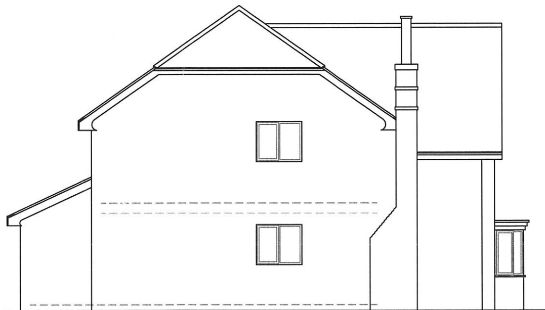
EXISTING SIDE HIPPED ELEVATION 'B'
